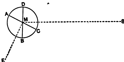
FIG. 8.—The phases of the moon.
