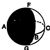
FIG. 9.—The phases of the moon.
