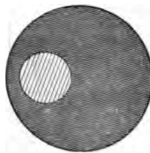
FIG. 29.—Total eclipse of the moon.
