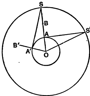
Fig. 39.—The daily rotation of the earth.
