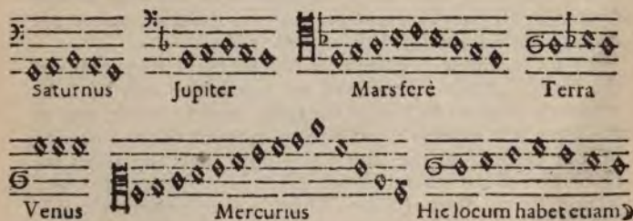
FIG. 62.—The “music of the spheres,” according to Kepler. From the Harmony of the World .
