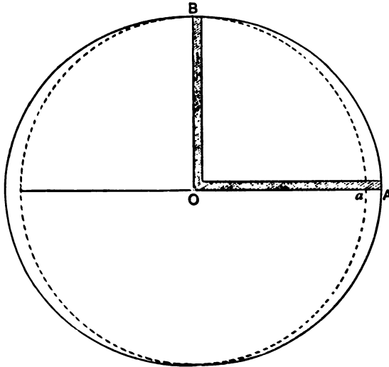
FIG. 72.—The spheroidal form of the earth.
