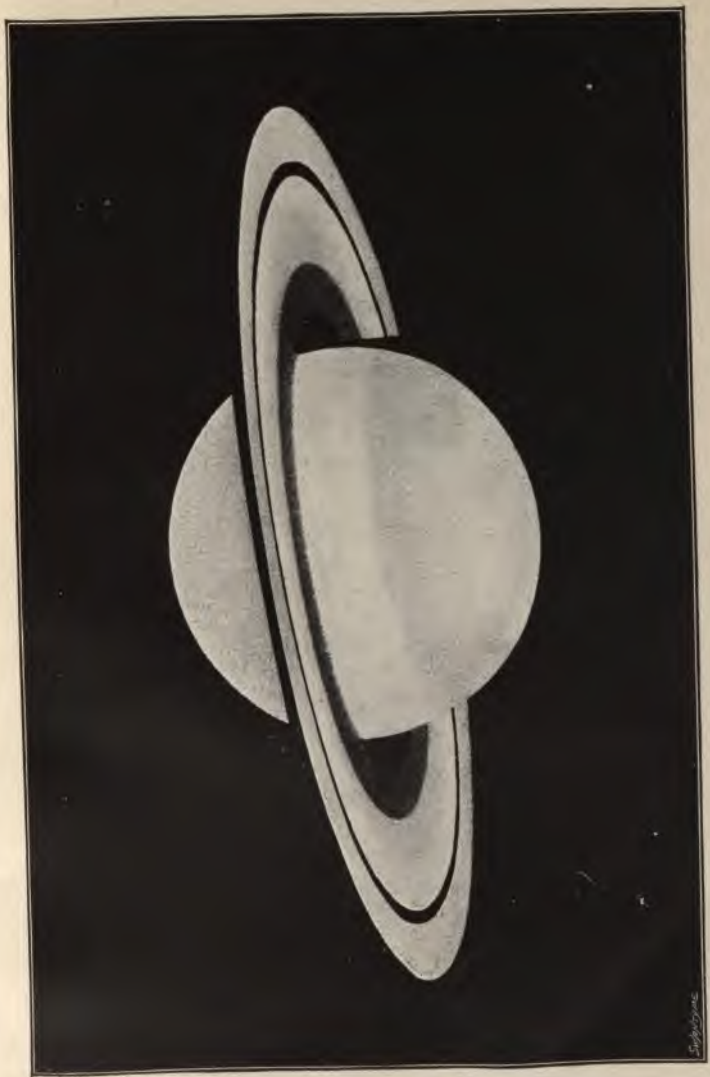
FIG. 95.— Saturn and its rings. From a drawing by Professor Barnard. [To face p. 384.
