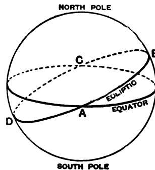
FIG. 4.—The equator and the ecliptic.
