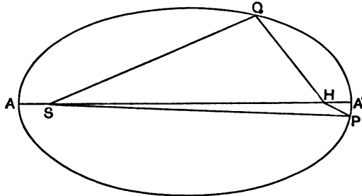
FIG. 59.—An ellipse.
