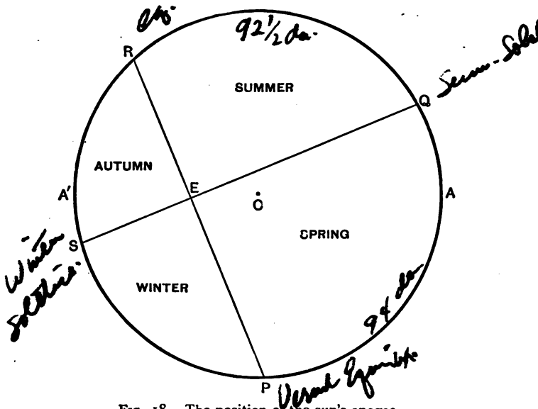
FIG. 18.—The position of the sun's apogee.
