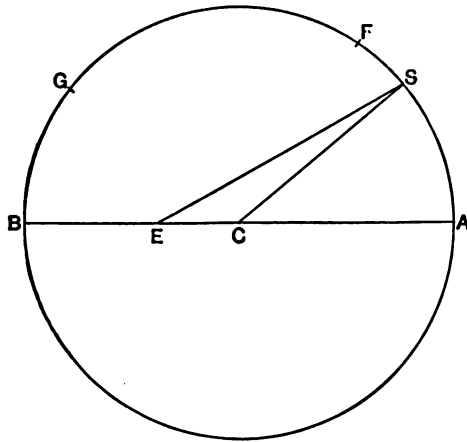
FIG. 17.—The eccentric.
