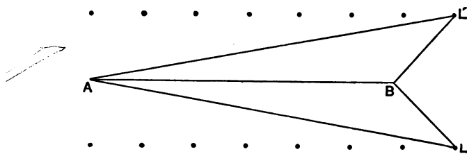
FIG. 84.—Illustrating the effect of the sun's motion in space.
