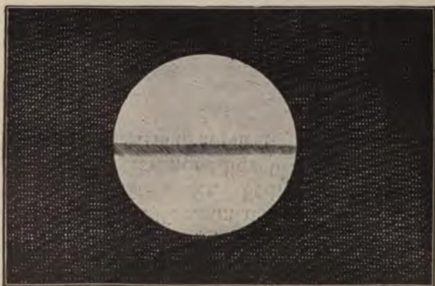
FIG. 65.—Saturn, with the ring seen edge-wise. From the Systema Saturnium . (To face p. 255)
