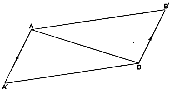
FIG. 37.—Relative motion.
