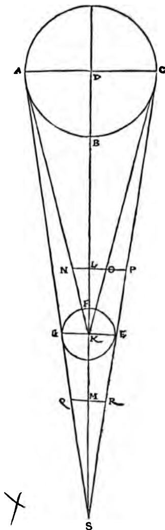
FIG. 20.—The eclipse method of connecting the distances of the sun and moon.
