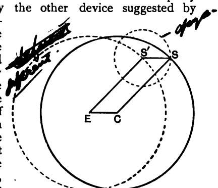
FIG. 19.—The epicycle and the deferent.
