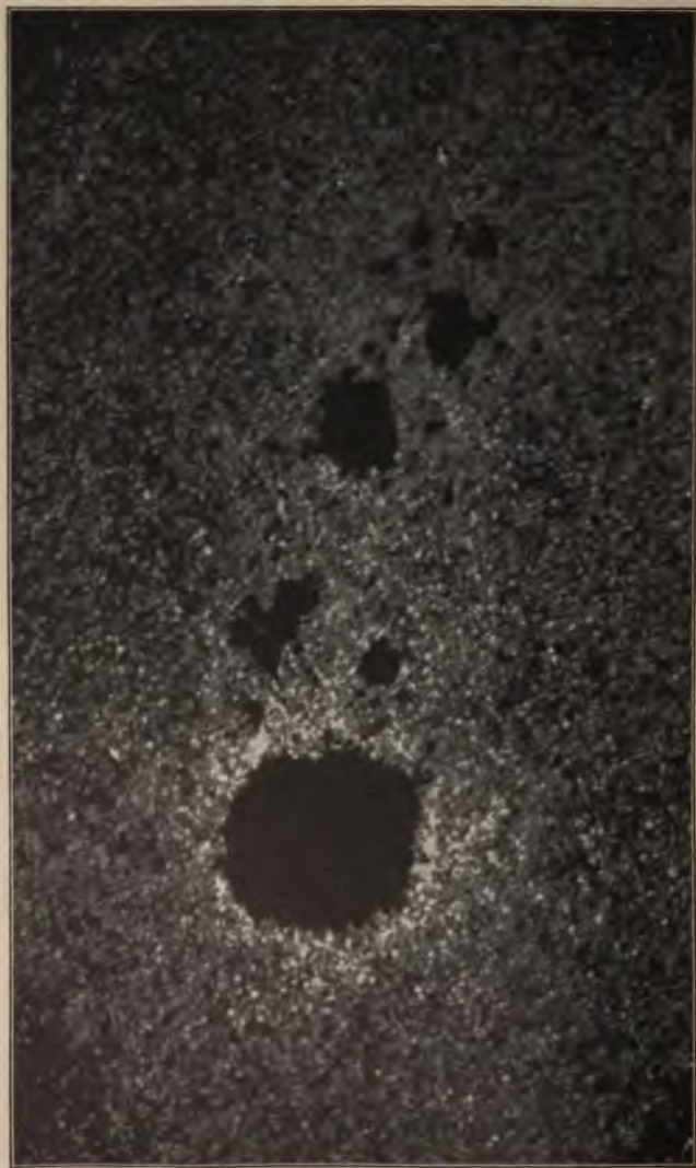
FIG. 96.—A group of sun-spots. From a photograph taken by M. Janssen at Meudon on April 1st, 1894. (The face of the sun.)
