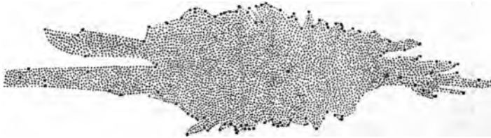
FIG. 83.—Section of the sidereal system. From Herschel's paper in the Philosophical Transactions .
