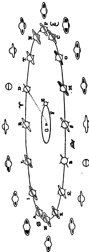
FIG. 66.—The phases of Saturn's ring From the Systema Saturnium .
