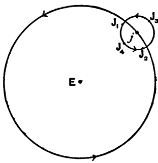
FIG. 34.—Jupiter's epicycle and deferent.
