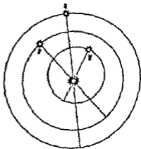
[454] Schemas of the Earth, Venus, and Mercury with orbit of the Earth enlarged
