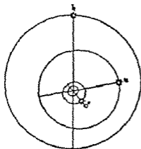
Schemas of Saturn, Jupiter, Mars, and the Earth
